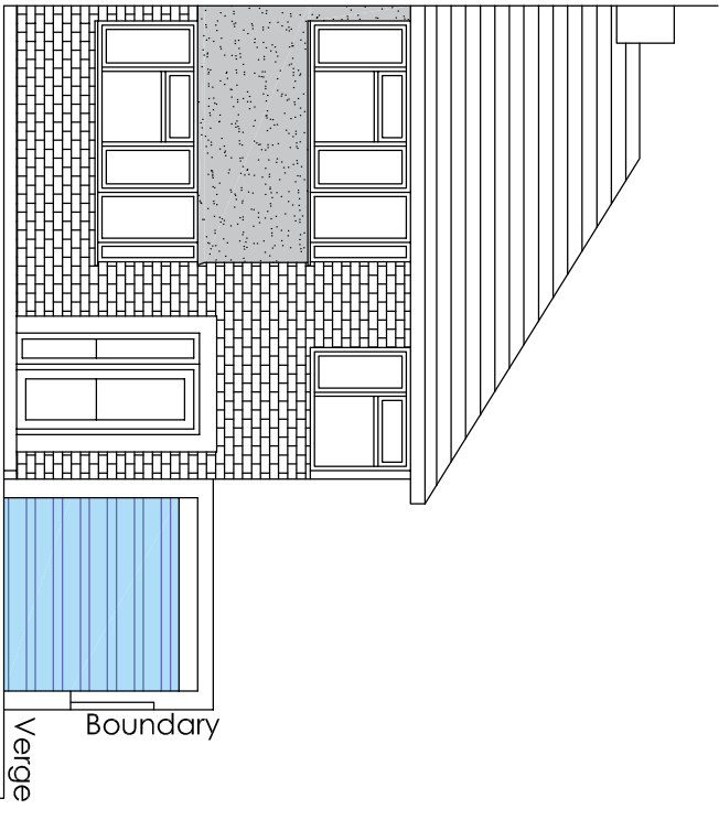
Front Elevation
