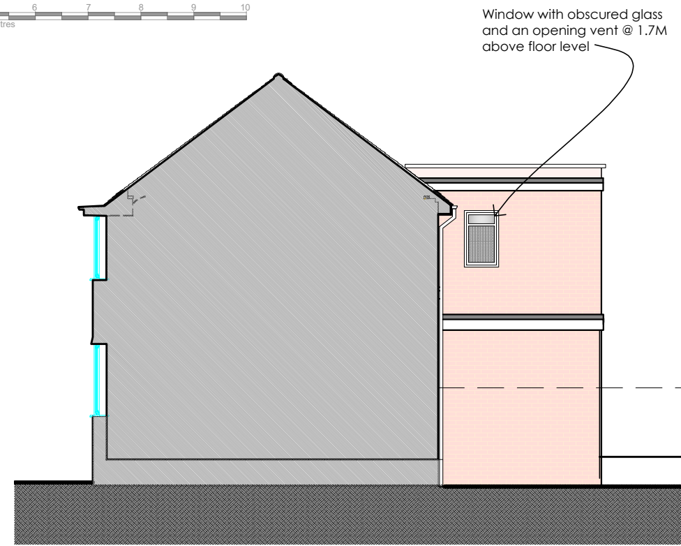
PROPOSED SIDE ELEVATION (NORTH)
