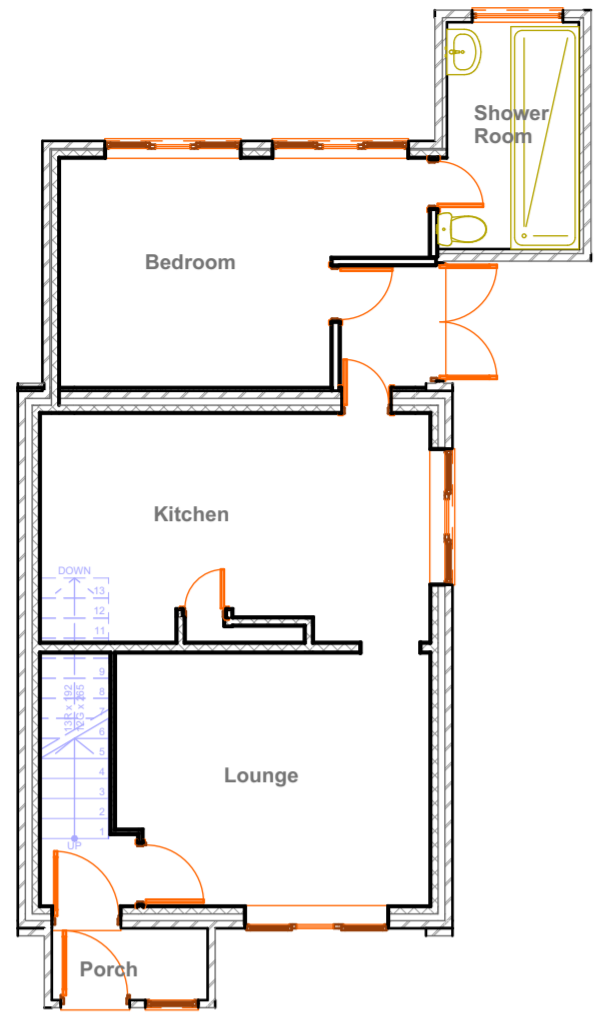
9 Existing Ground Floor 1:100
