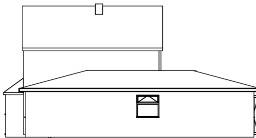
5 Proposed North Elevation 1:200
