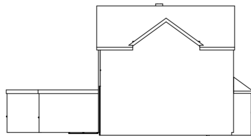
6 Proposed South Elevation 1:200
