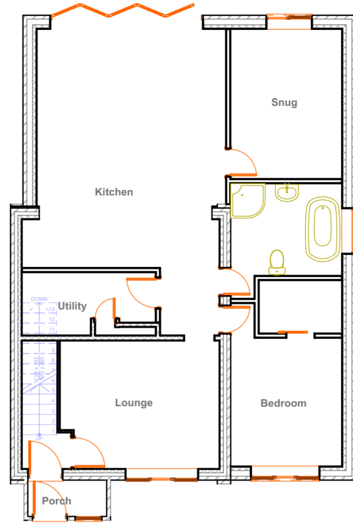
11 Proposed Ground Floor 1:100
