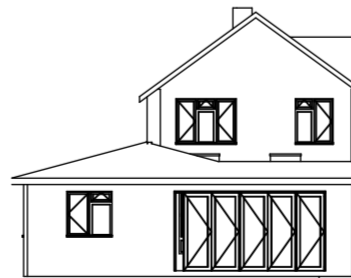
8 Proposed West Elevation 1:200
