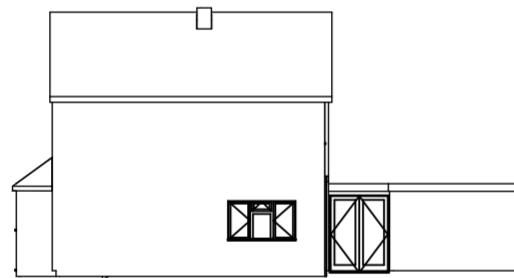
1 Existing North Elevation 1:200
